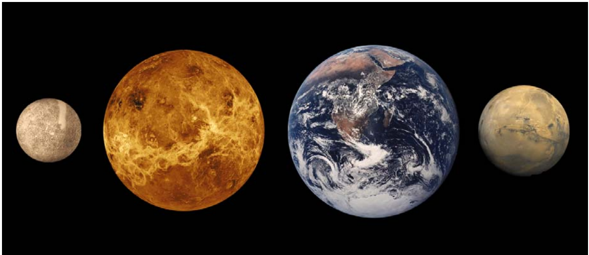
Mercury, Venus, Earth, and Mars to scale
