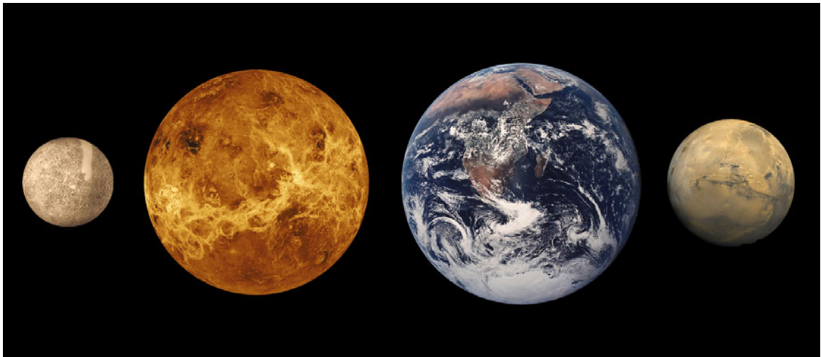
Mercury, Venus, Earth, and Mars to scale
